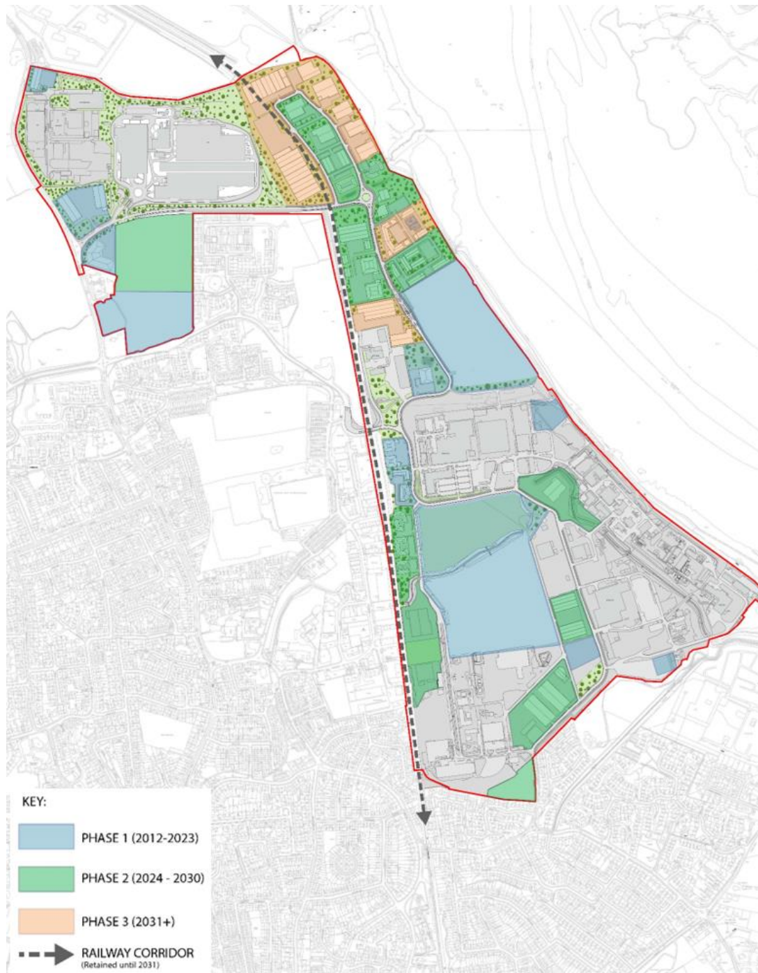
Figure 11: Phasing plan
